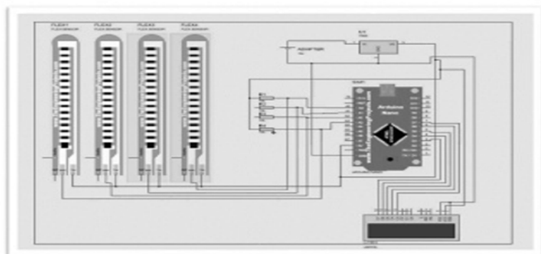
Fig 1: Circuit Diagram of the device
