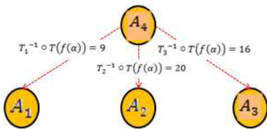
Figure 11. Transmission of signals from A_4 to the other users for key retrieving
