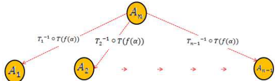
Figure 5. Transmission of signals from A_n to the other users for key retrieving
